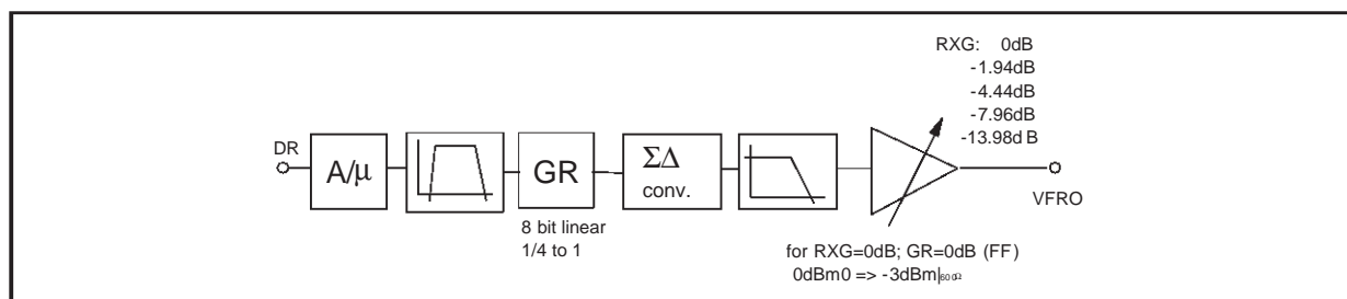
Figure 2. Receive path.
